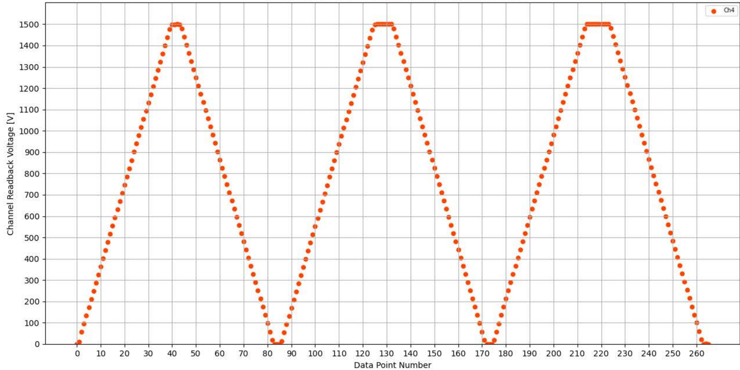
Voltage Ramp Test (Python) Bd #128, Slot #1, Ch #4
