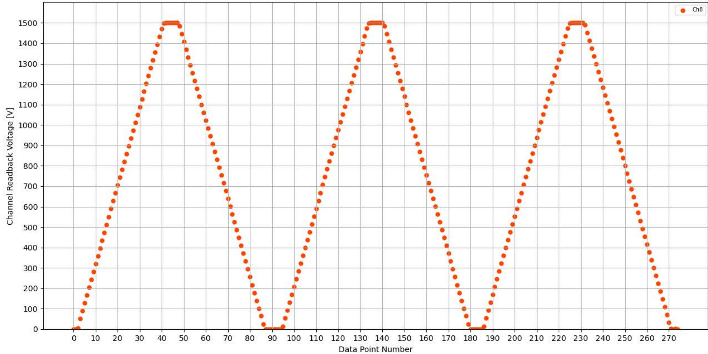
Voltage Ramp Test (Python) Bd #128, Slot #1, Ch #8
