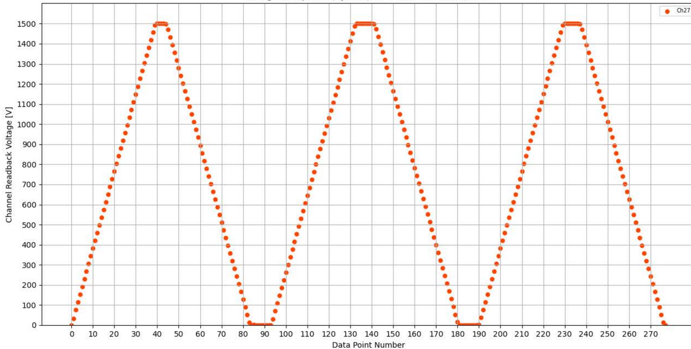
Voltage Ramp Test (Python) Bd #128, Slot #1, Ch #27
