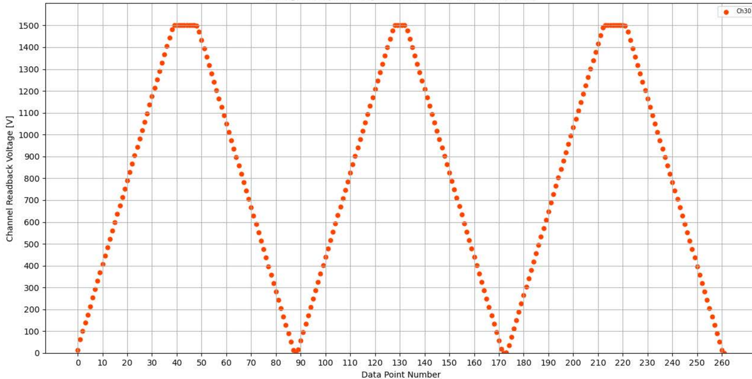
Voltage Ramp Test (Python) Bd #128, Slot #1, Ch #30
