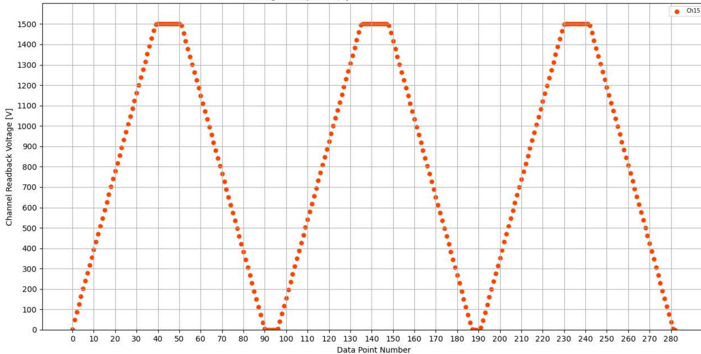
Voltage Ramp Test (Python) Bd #128, Slot #1, Ch #15
