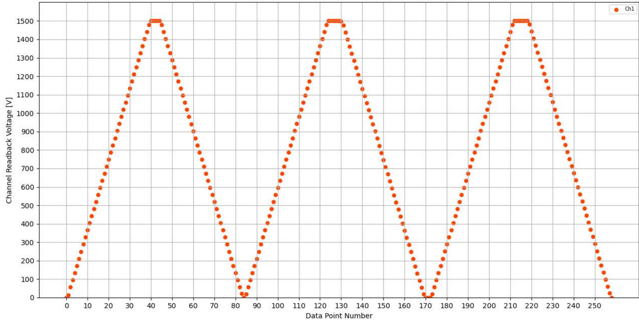
Voltage Ramp Test (Python) Bd #128, Slot #1, Ch #1
