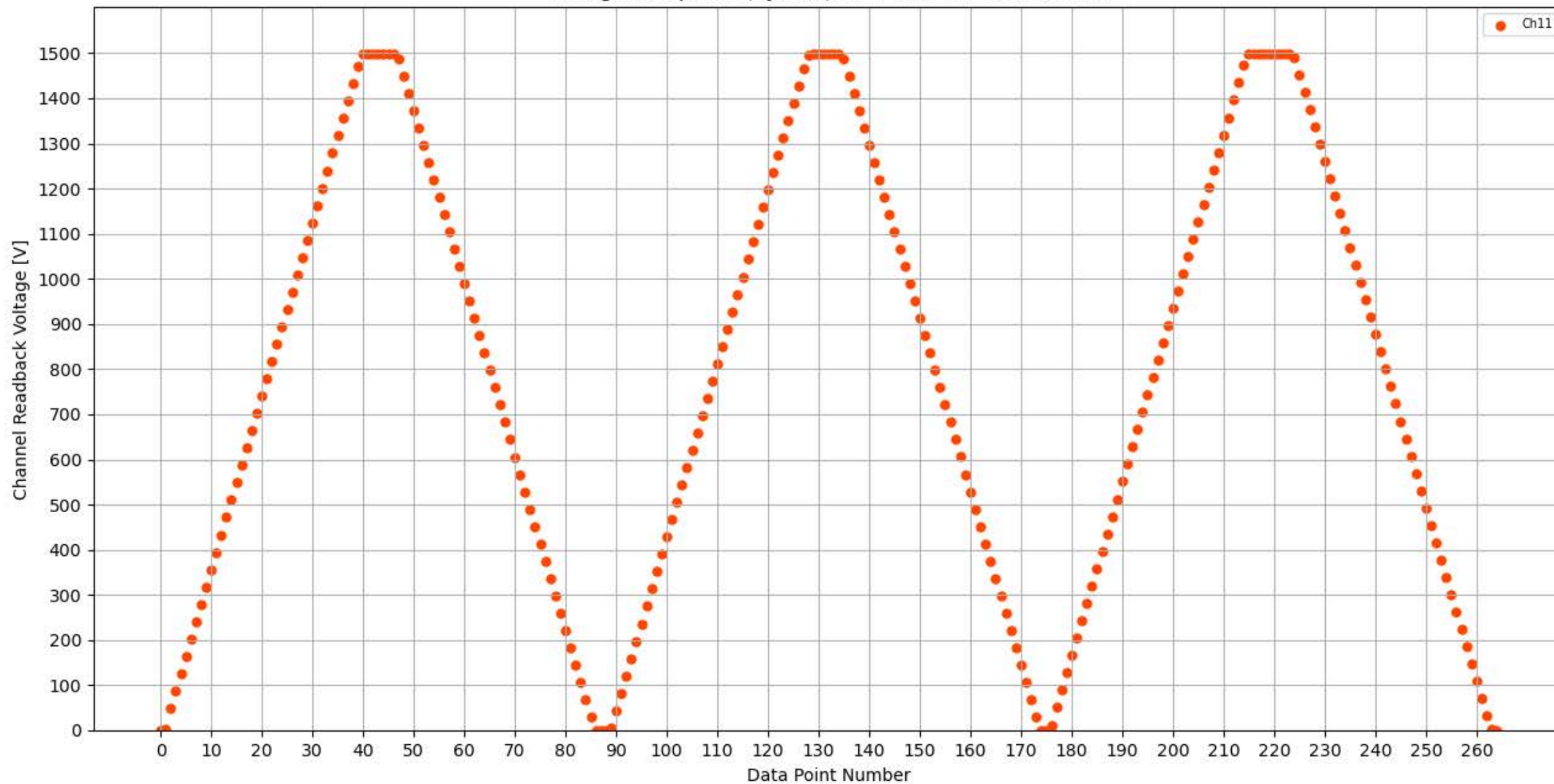
Voltage Ramp Test (Python) Bd #128, Slot #1, Ch #11
