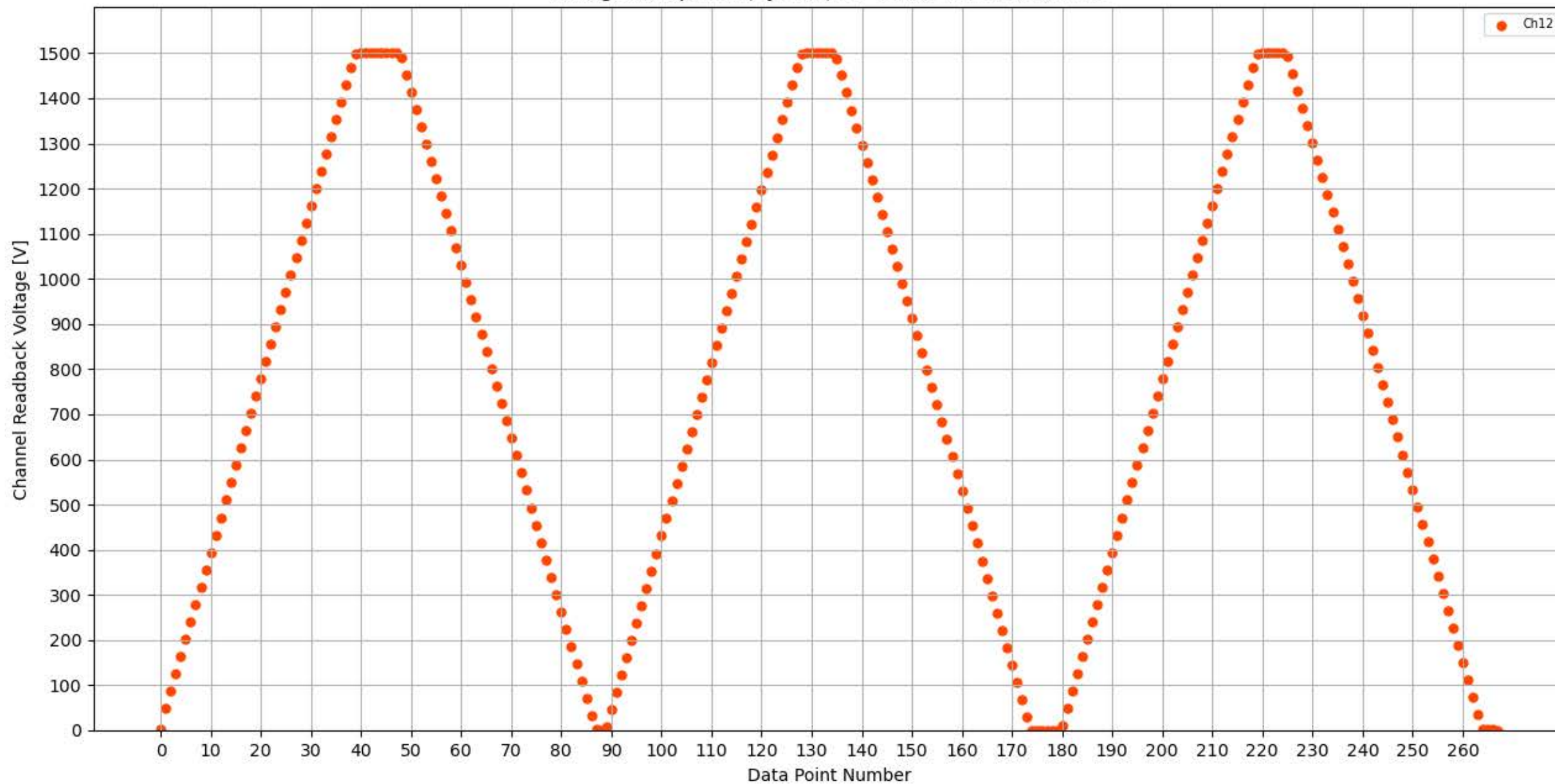
Voltage Ramp Test (Python) Bd #128, Slot #1, Ch #12
