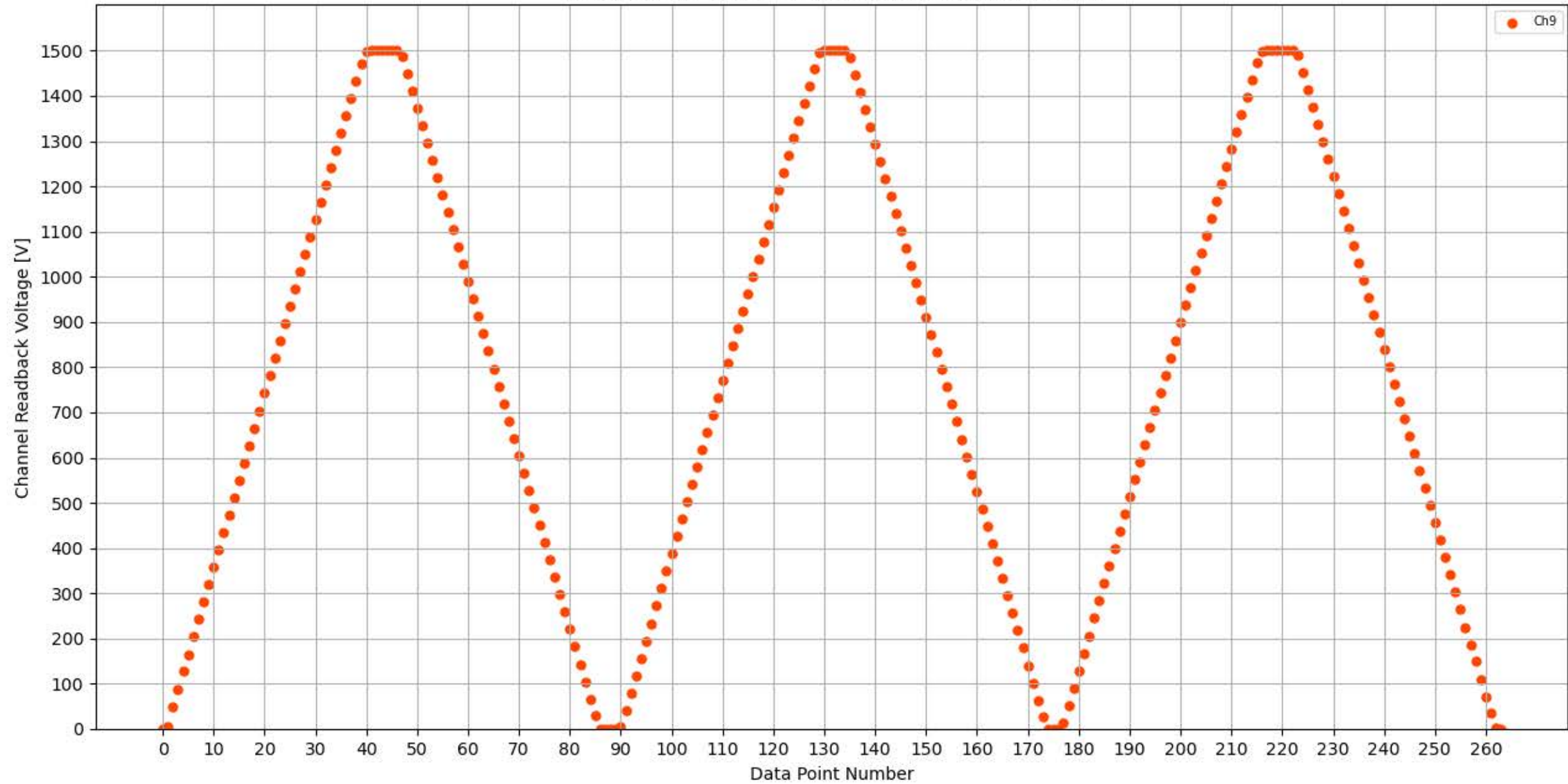
Voltage Ramp Test (Python) Bd #128, Slot #1, Ch #9
